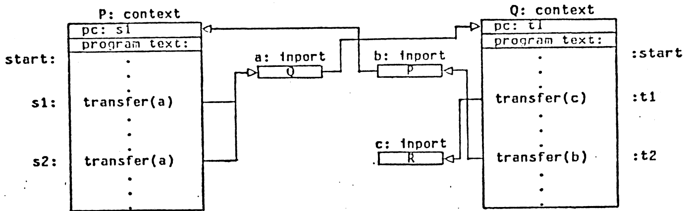
Figure 1: Coroutine linkages
